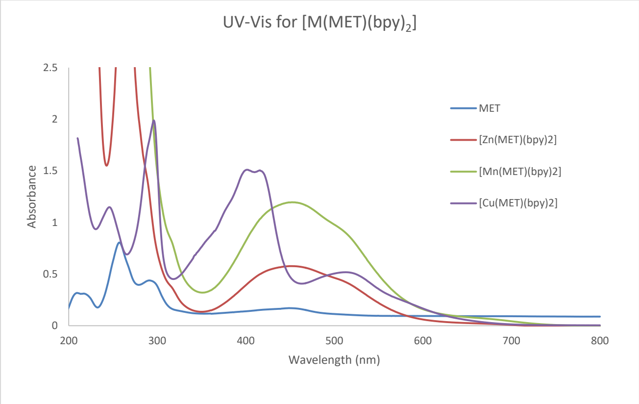
Figure 2. Electronic Spectra of synthesized complexes
